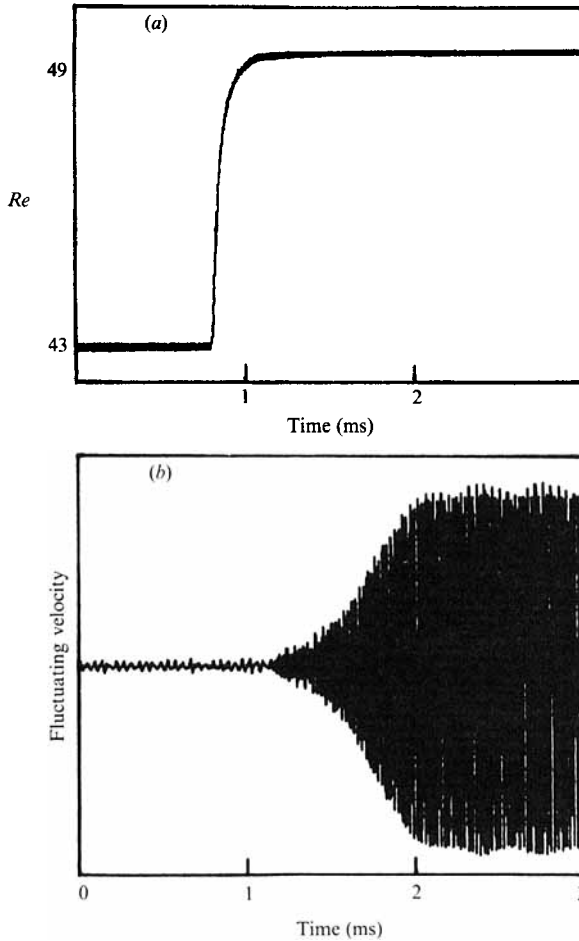
FIGURE 15. Simultaneous records of the mean and fluctuating velocities. The flow Reynolds number was increased from 43 to 49 (the critical Reynolds number, Re_{cr} , being 46 in this instance). Trace (a) was low-pass filtered below 30 Hz, and trace (b) was high-pass filtered above 30 Hz.
