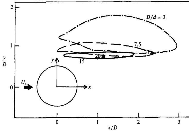
FIGURE 5. Regions of suppression for four values of D/d . These regions are symmetrical about the plane y = 0 . Re = 80 .
