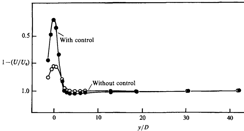
FIGURE 10. Mean velocity distribution 1 - (U/U_0) at x/D = 58 , D/d = 8.5 and Re = 65 . Notice the long tail for the case with suppressed shedding.
