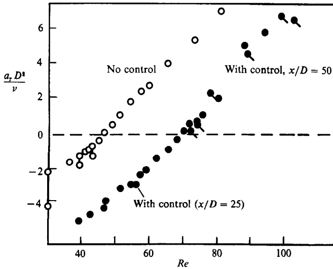
FIGURE 21. Amplification and decay rates in the wake with and without control. The control cylinder was located at x/D = 1.2 and y/D = 0.95 ; D/d = 10 .
