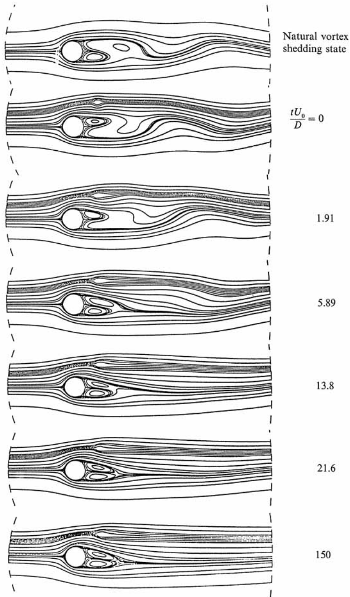
FIGURE 13. Instantaneous streamline pattern indicating the effect of the control cylinder at Re = 55 . The uppermost figure represents the natural case at the same Reynolds numbers as the rest. The remaining figures correspond to increasing values of tU_0/D . The control 'cylinder' is located as indicated in figure 12.
