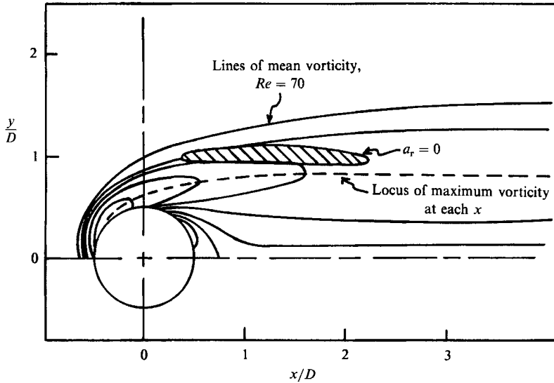
FIGURE 28. Mean vorticity lines plotted with the contour a_r = 0 at Re = 70 . The mean vorticity data are for steady flow at Re = 70 from Dennis & Chang (1970).
