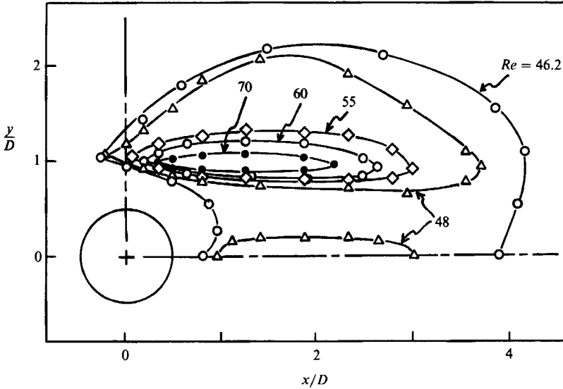
FIGURE 20. Contours where a_r = 0 for several Reynolds numbers. Data are symmetric about the line y = 0 ; D/d = 10 .
