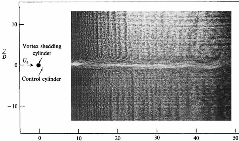
FIGURE 3. Hydrogen-bubble picture showing the control of vortex shedding at Re = 80 using a control cylinder of D/d = 7 .
