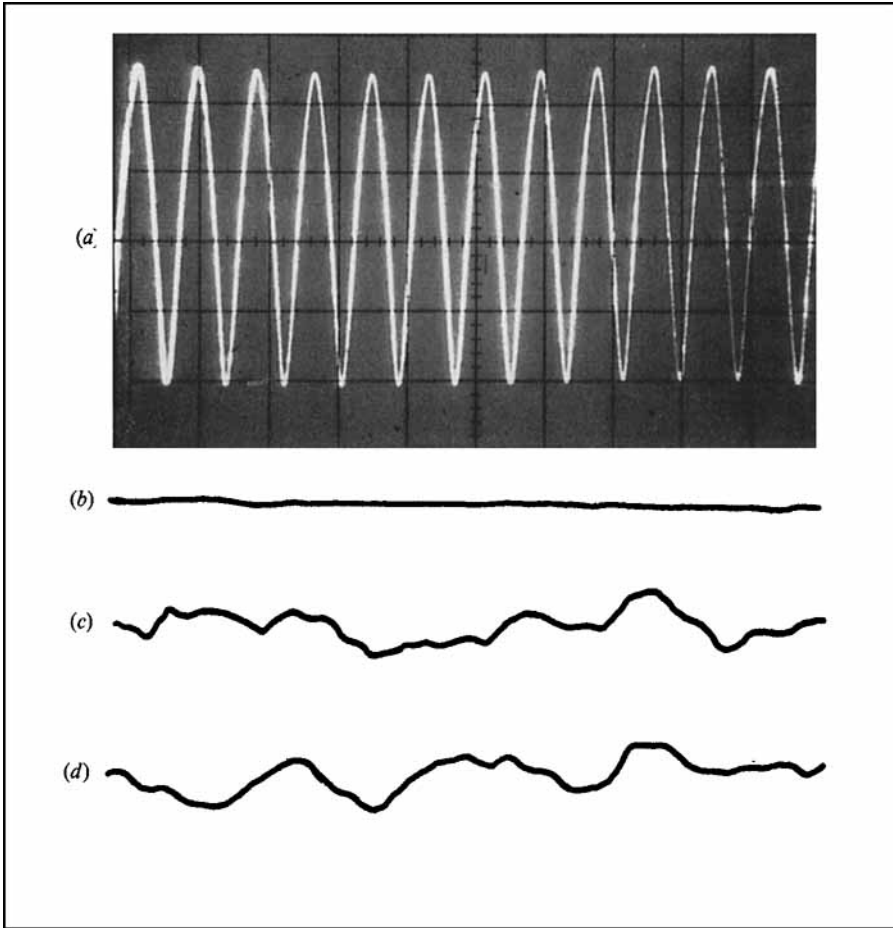
FIGURE 4. Hot-wire oscillations in the wake with and without control at Re = 71 . (a) x/D = 10 and y/D = 1 , no control; (b) x/D = 10 and y/D = 1 , with control, D/d = 11 ; (c) same as (b), except for an amplification of about 20; (d) x/D = 100 , all other conditions remaining the same as in (c). There is typically some small amplification of the disturbances between x/D of 10 and 100.
